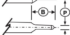
FIG. 2C STEPPED PILOT NOSE
