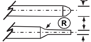
FIG. 1A STRAIGHT PILOT NOSE
